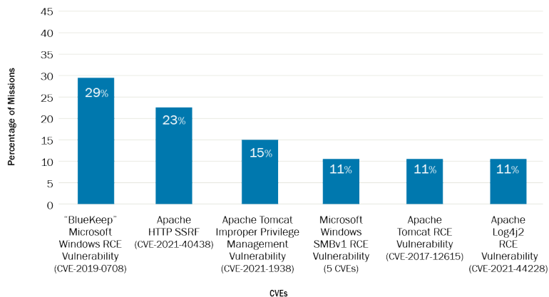
Figure 9: Top KEV Detected During CY22 Assess Missions
