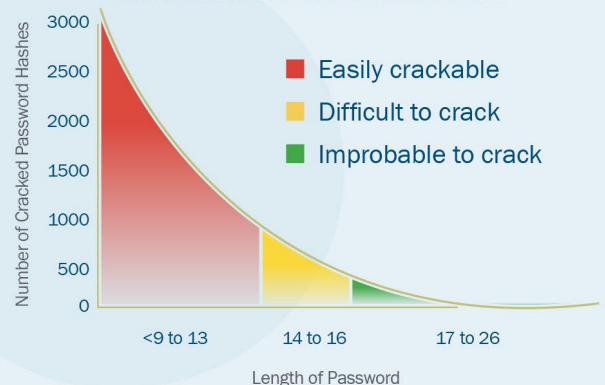
Length of Cracked Password Hashes from CY22 Missions
