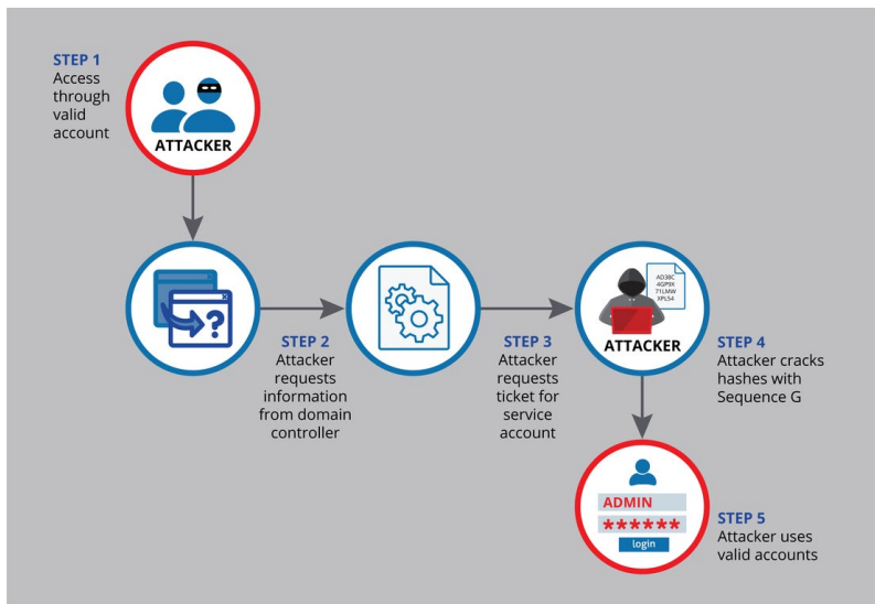
Figure 8: Kerberoasting
