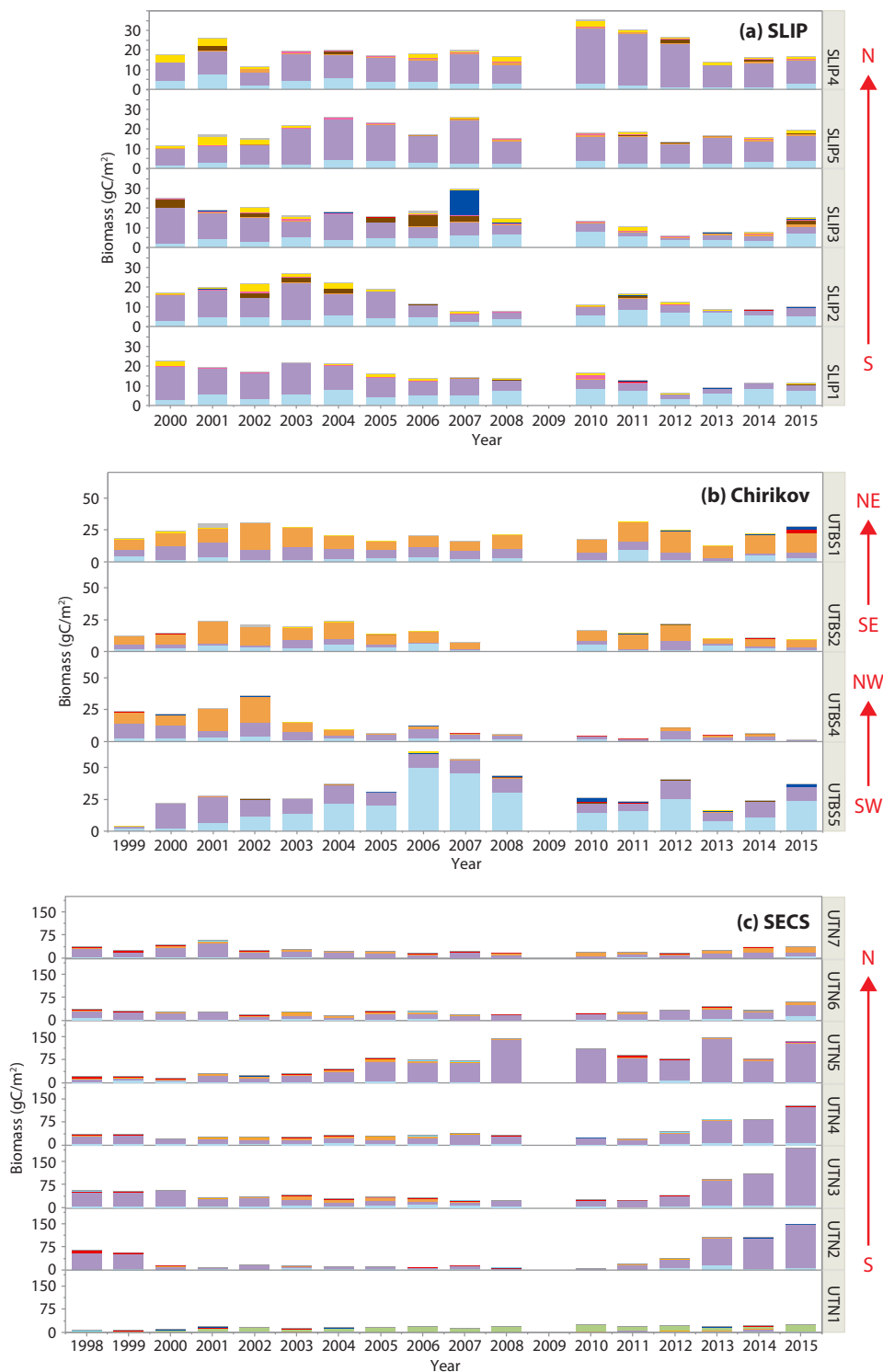
FIGURE 4. Time series histograms of macrofaunal biomass (gC/m²) for the different taxa at each station for the three regions: (a) SLIP, stations SLIP1–SLIP5. (b) Chirikov, stations UTBS1, UTBS2, UTBS 4, UTBS 5. (c) SECS, stations UTN1–UTN7. Colors designate the dominant faunal type: polychaetes (light blue), bivalves (lavender), and crustaceans (amphipods) (orange). Remaining taxa are color keyed. The red arrows indicate the general location of stations from South (S) to North (N) within each of the SLIP and SECS regions. The Chirikov region has four time series sites located Southwest (SW), Northwest (NW), Southeast (SE), and Northeast (NE) in the region. See Figure 1 for the spatial location of the time series regions and stations.
