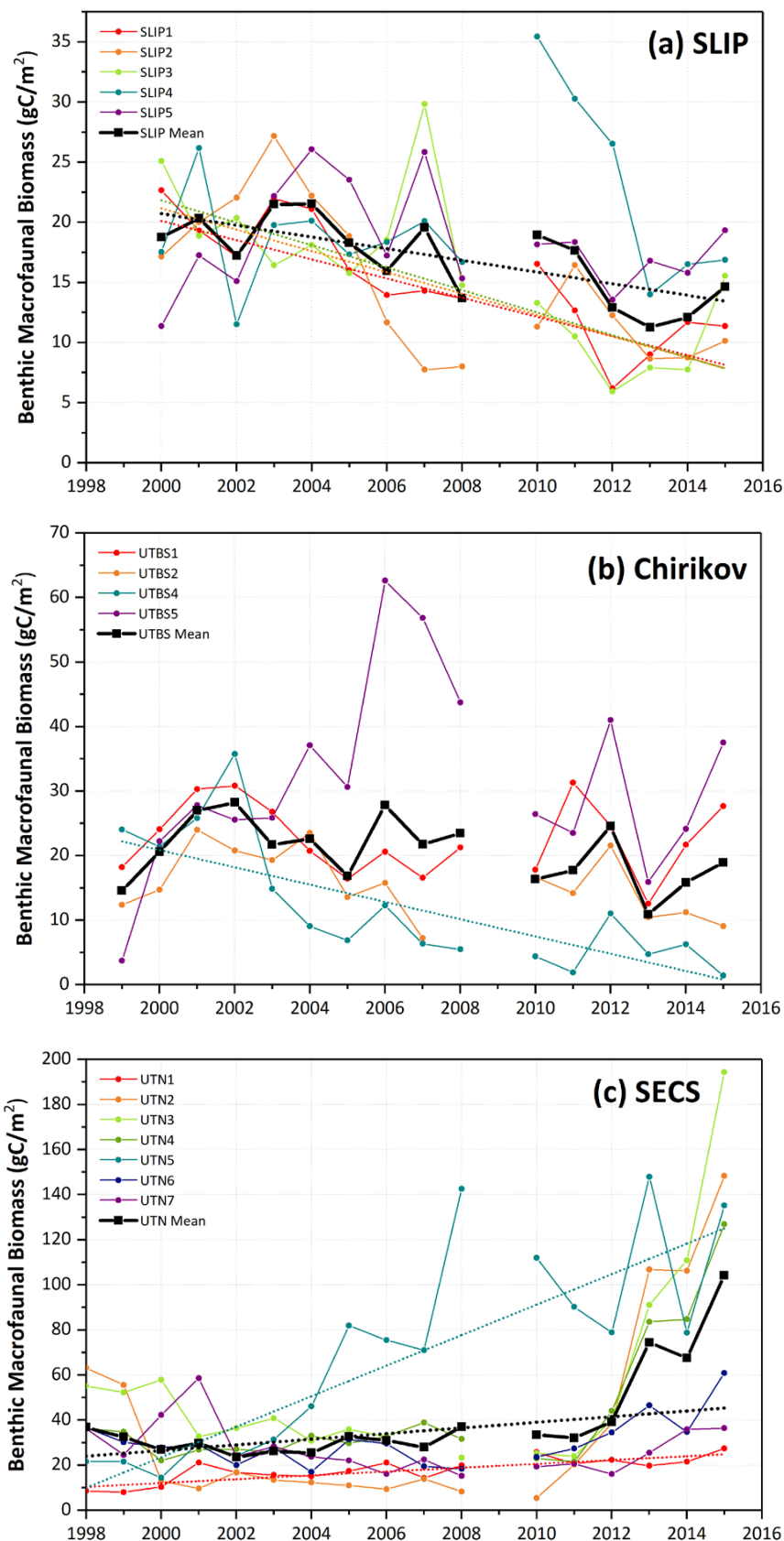
FIGURE 3. Time series data of individual station benthic biomass (gC/m 2 ) as well as averages for the three regions over similar time periods: (a) SLIP, 2000–2015, (b) Chirikov, 1999–2015, and (c) SECS, 1998–2015. Sen's median slope estimators are shown only for those time series that show statistically significant trends (Mann-Kendall test for trend, p < 0.05 ), with statistics provided in Table 3. Note the increasing biomass scale from the SLIP region (south) to the SECS region (north). No July field program occurred in 2009.
